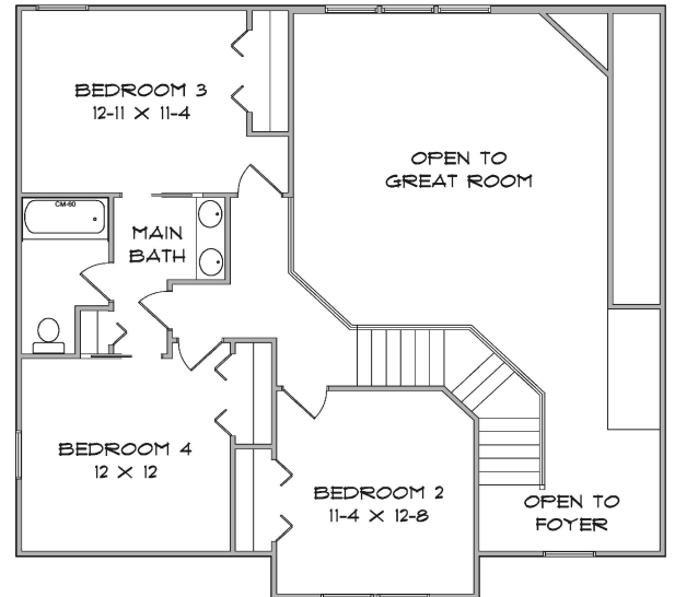
Second Floor Plan 720 Sq Ft
