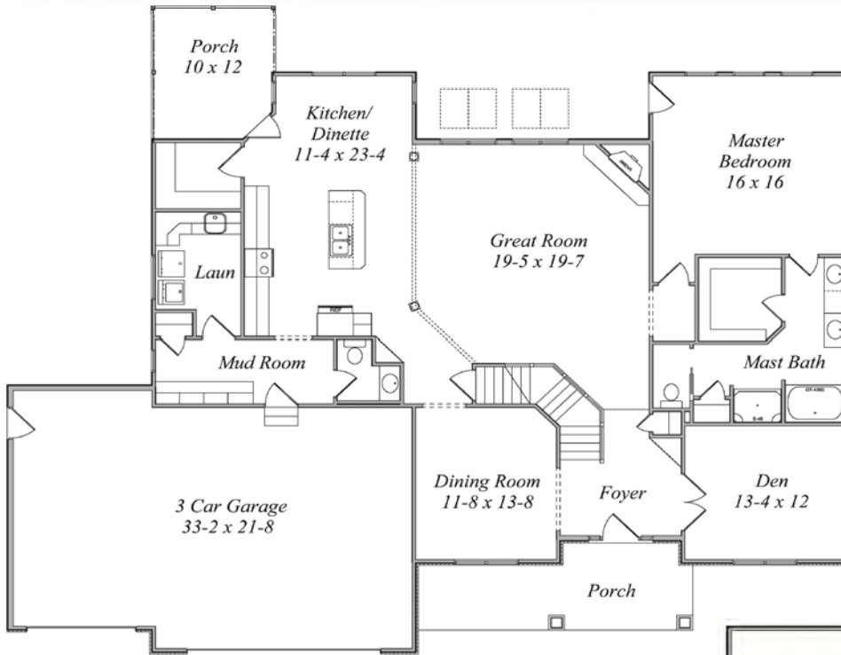
First Floor Plan 2055 Sq Ft
